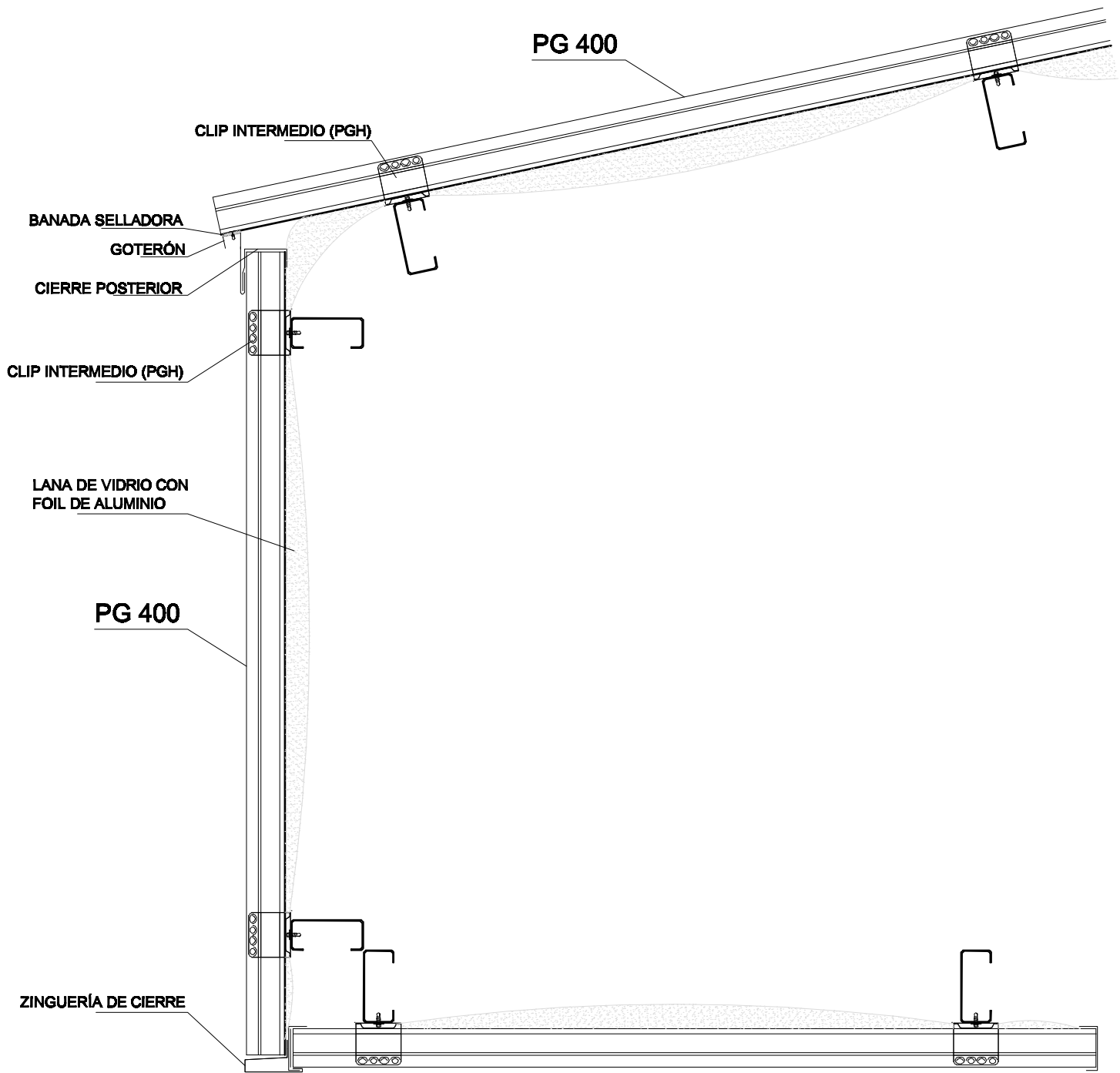
DETALLE FRENTIN PG400
